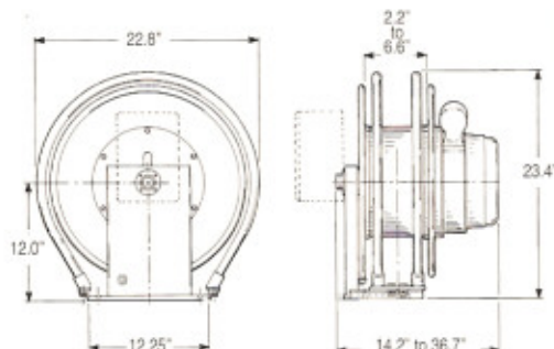
Hazardous location option includes fully enclosed junction boxes
